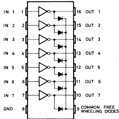
Figure 6.7. Pinout for the ULN2003.
