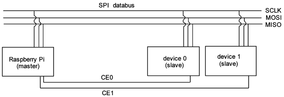
Figure 8.2. Basic SPI configuration with two slaves.
