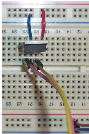
Figure 9.14. Setup on the breadboard.
