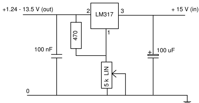
Figure A.1. Circuit for the adjustable power supply.
