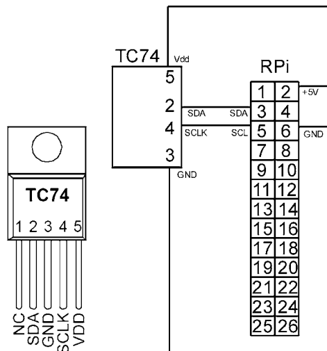
Figure 9.13. Connecting the TC74, note the +5 V pin.
