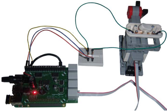
Figure 14.9. The complete model.
