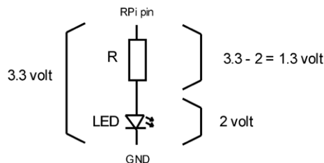
Figure 5.2. Working out the current limiting resistor.
