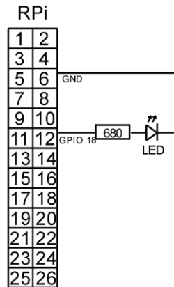
Figure 7.3. Connection to the PWM pin on the header.
