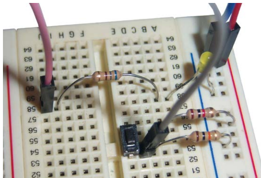
Figure 11.12. Setup on the breadboard.
