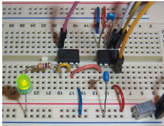
Figure 8.12. Setup on the breadboard.
