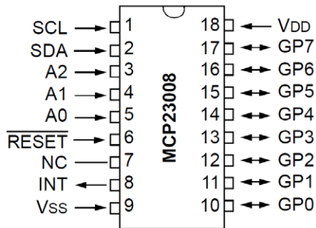
Figure 9.6. Pinout for the MCP23008.
