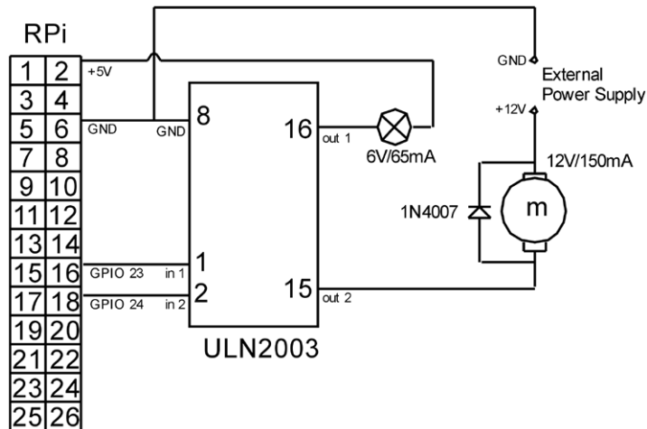
Figure 6.9. Controlling devices with different operating voltages.
