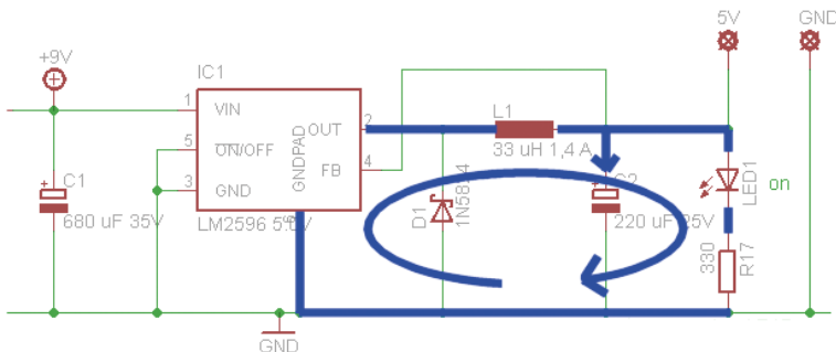
Figure 14.3. Buck converter: starting the flywheel.
