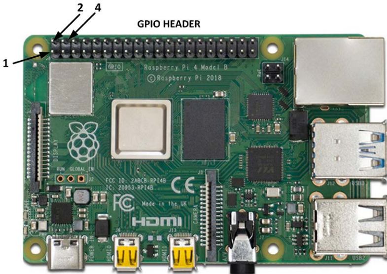
Figure A.4. The header on the Raspberry Pi.
