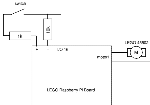
Figure 14.8. Connection diagram.
