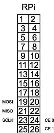
Figure 8.1. SPI pins on the header.
