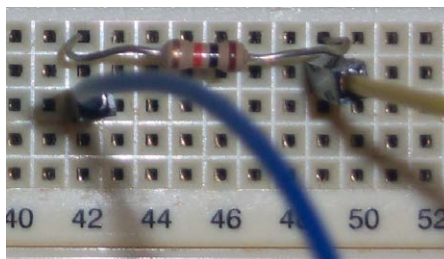
Figure 5.15. Connections on the breadboard.
