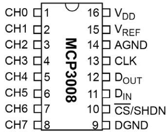
Figure 8.15. Pinout for the MCP3008.
