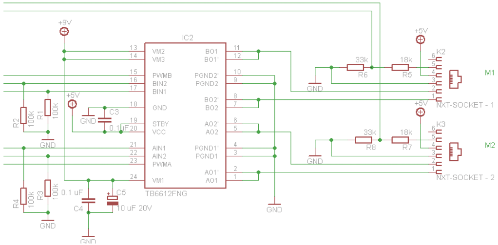
Figure 14.6. LEGO Raspberry Pi board motor driver (M1 and M2).
