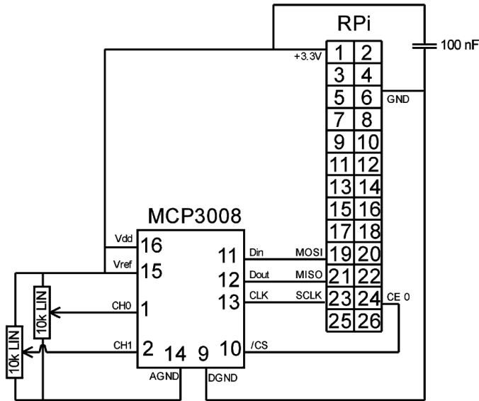
Figure 8.16. Connection of the MCP3008 to the header.
