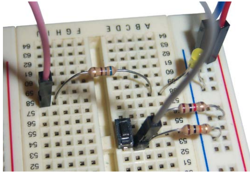
Figure 5.12. Setup on the breadboard.
