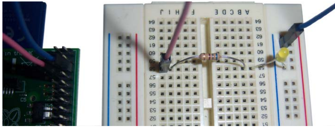
Figure 5.5. The setup on the breadboard.
