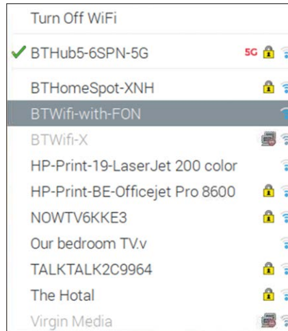
Figure 2.12 WiFi options
