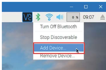
Figure 2.11 Bluetooth options
