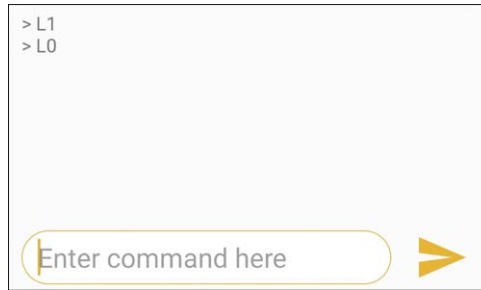
Figure 13.3 Mobile application
