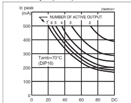
Figure 6.6. Output current versus duty cycle according to the datasheet.
