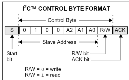
Figure 9.4. Address structure with pins A2:A0.
