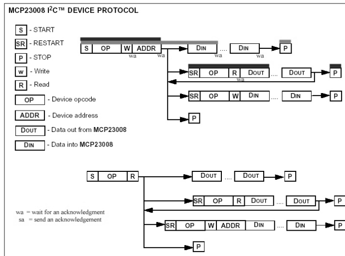
Figure 9.5. I 2 C device protocol for the MCP23008.
