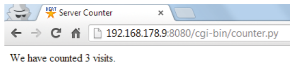
Figure 11.8. Visitor counter.
