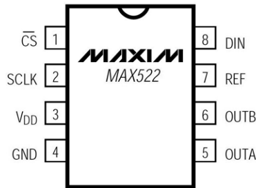
Figure 8.3. Pinout for the MAX522.
