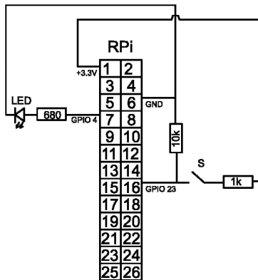
Figure 11.11. Connection of a switch and LED to the header.
