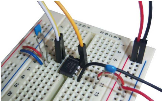
Figure 8.6. Setup on the breadboard.
