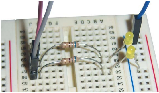
Figure 5.7. The setup on the breadboard.
