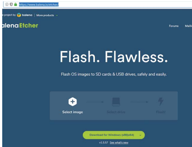
Figure 3.4 Download Etcher
