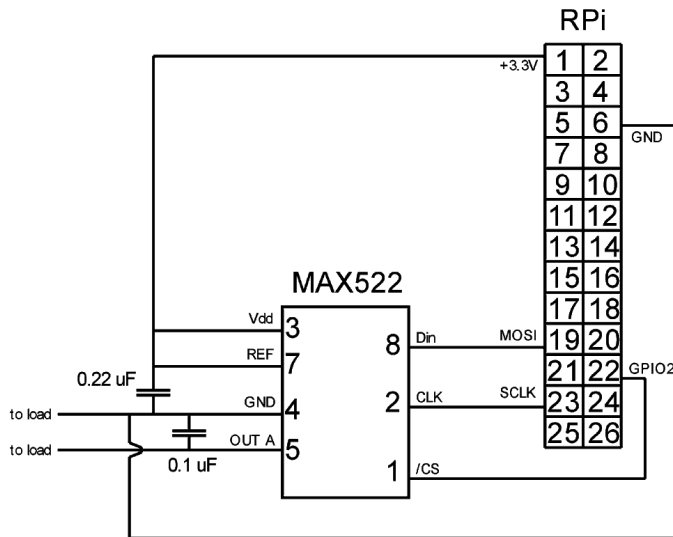
Figure 8.14. MAX522 connected to an "extra" CE pin.
