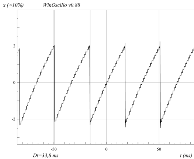
Figure 12.5. Sawtooth.
