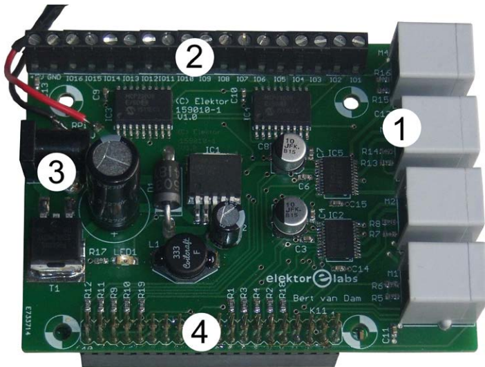
Figure 14.1. LEGO Raspberry Pi board.
