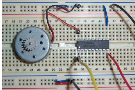
Figure 7.10. Setup with the motor on the breadboard.
