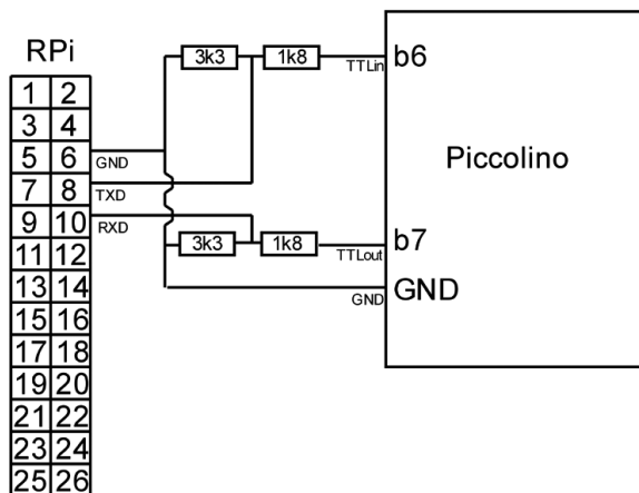
Figure 10.6. Connecting the Piccolino to the header of the Raspberry Pi.
