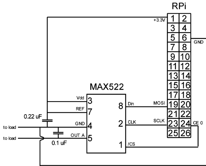
Figure 8.5. Connecting the MAX522 to the header.
