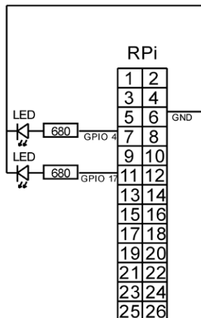
Figure 5.6. Connection of the LEDs to the header.
