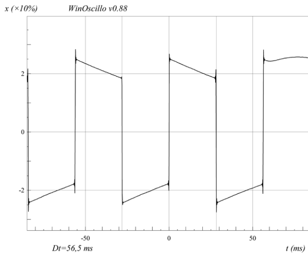
Figure 12.6. Square wave.
