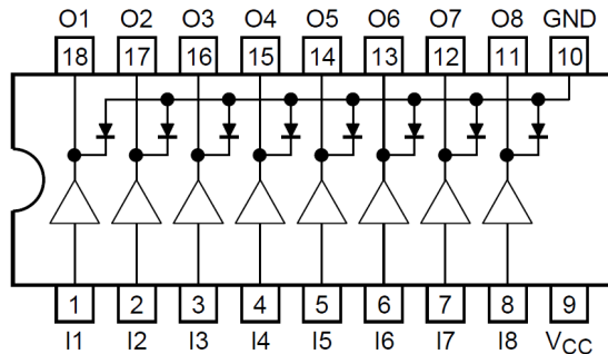
Figure 6.2. Pinout for the TD62783.
