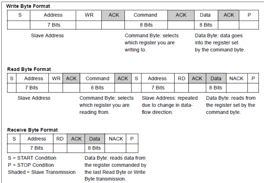
Figure 9.10. I 2 C communications according to the datasheet.
