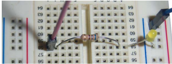
Figure 7.2. Setup on the breadboard.
