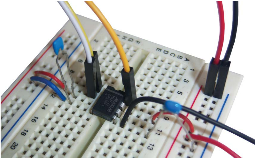
Figure 12.4. Setup on the breadboard.
