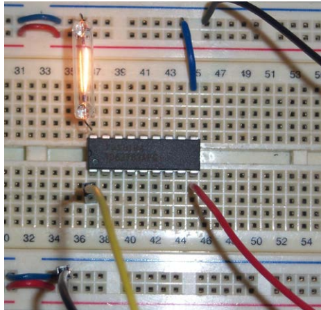
Figure 6.4. Setup on the breadboard.
