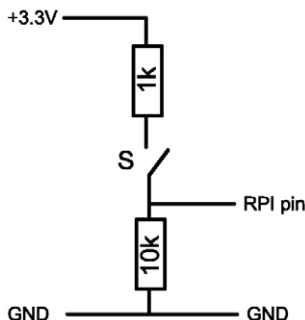
Figure 5.10. Protected switch connection for the Raspberry Pi.
