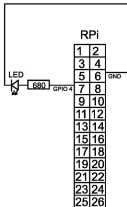
Figure 5.3. Connecting the LED to the header.
