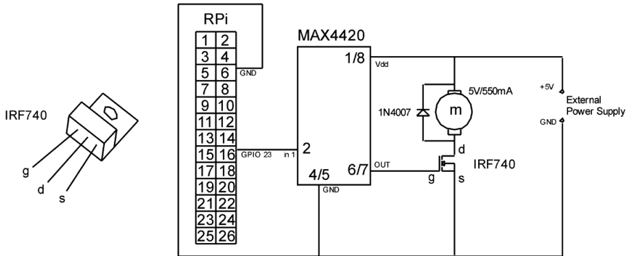
Figure 6.11. Connection of a motor and MOSFET to the header.
