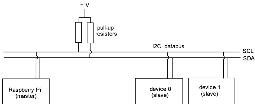
Figure 9.1. Basic I 2 C setup with two slaves.
