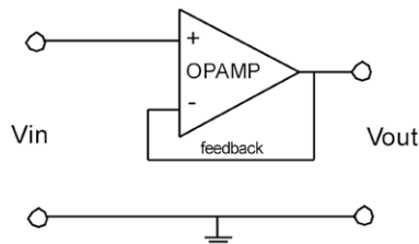
Figure 8.9. Opamp used as a non-inverting voltage follower.
