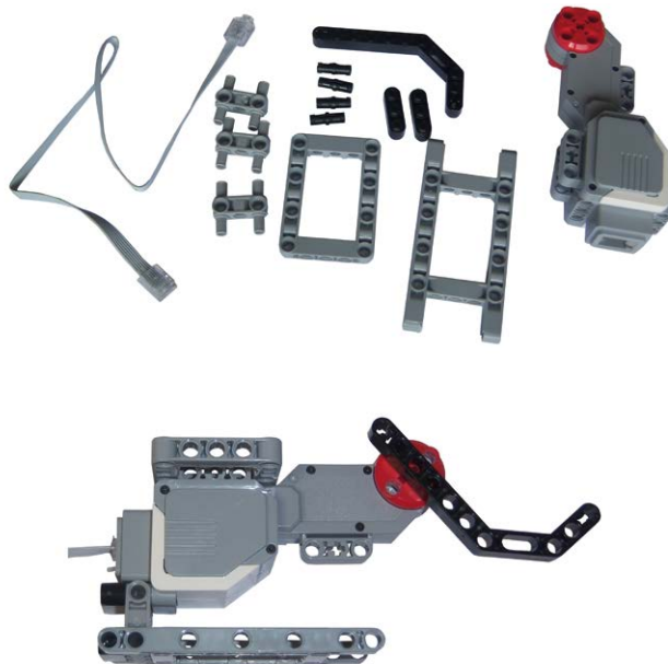
Figure 14.7. Parts for the motorized finger, and a completed model.
