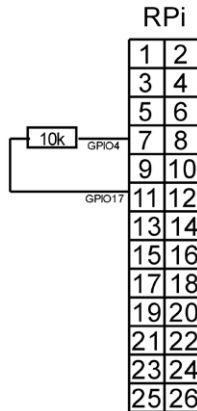
Figure 5.16. Connecting the pins on the header.
