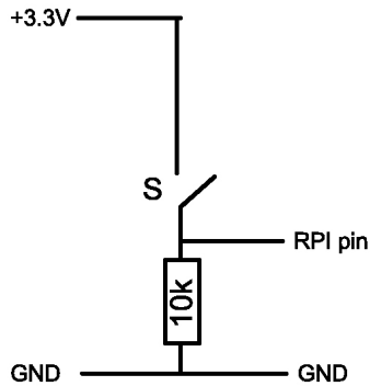
Figure 5.9. Standard switch connection.
