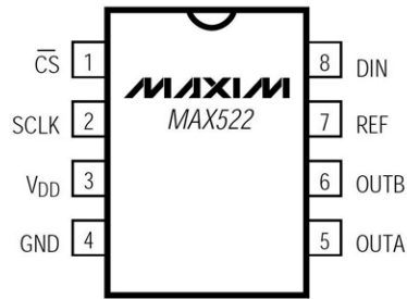
Figure 12.2. Pinout for the MAX522.
