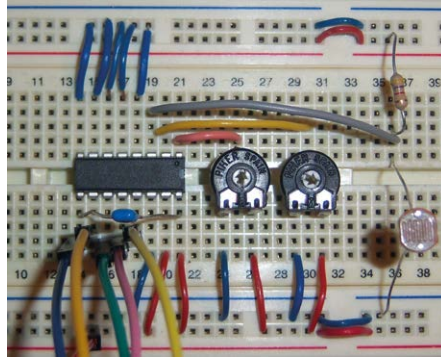
Figure 12.10. Setup on the breadboard.
