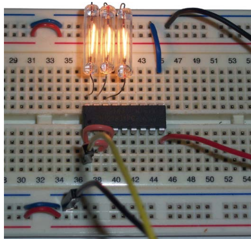
Figure 7.8. Setup on the breadboard.
