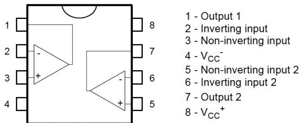
Figure 8.10. Pinout for the LM358 opamp.
