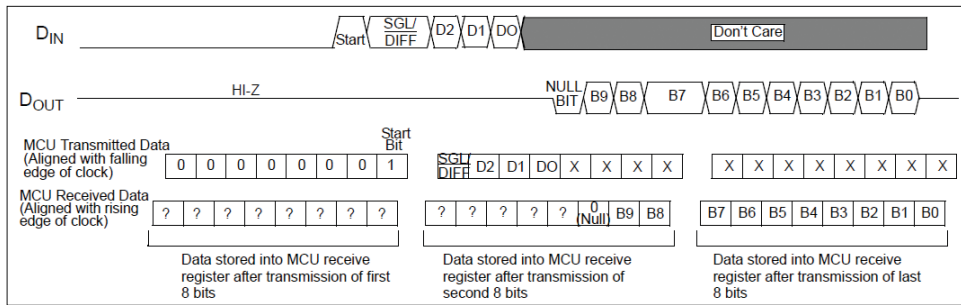
Figure 8.18. SPI communications according to the datasheet for the MCP3008.
