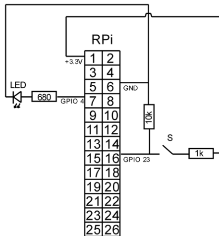
Figure 5.11. Connection of an LED and switch to the header.
