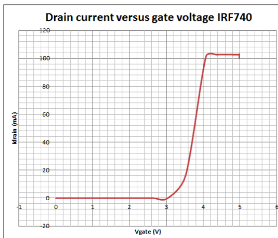
Figure 6.10. Drain current versus gate voltage for the IRF740.
