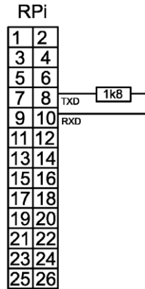
Figure 10.2. Serial loop with 1k8 resistor.
