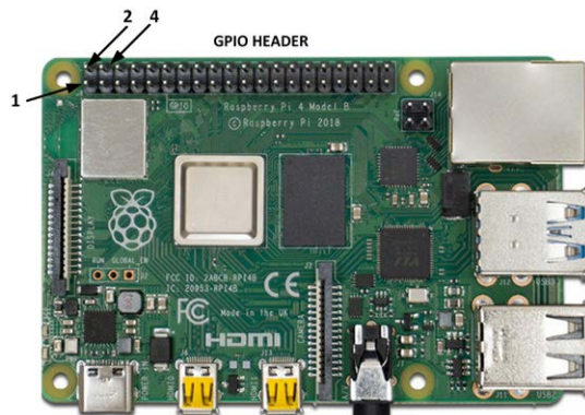
Figure 5.1. GPIO header on the Raspberry Pi 4
