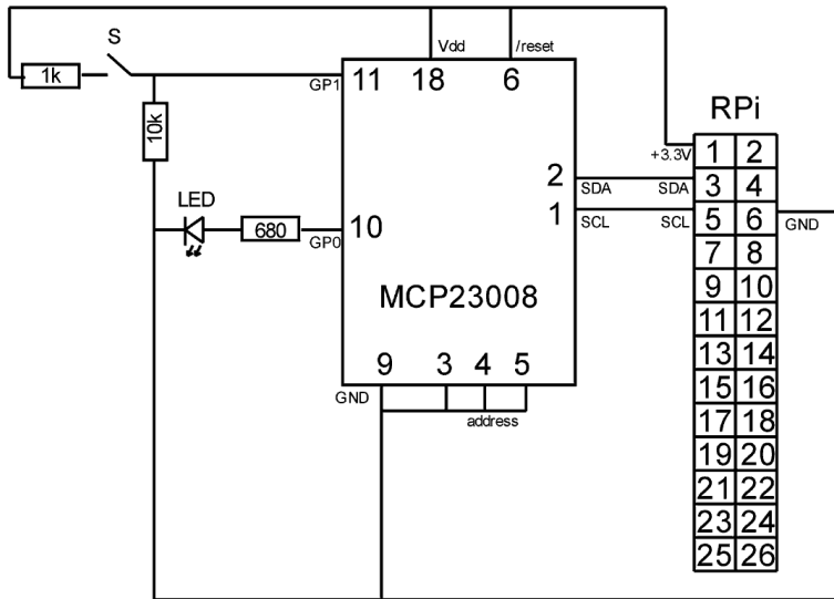
Figure 9.7. Circuit for the de I/O expander.
