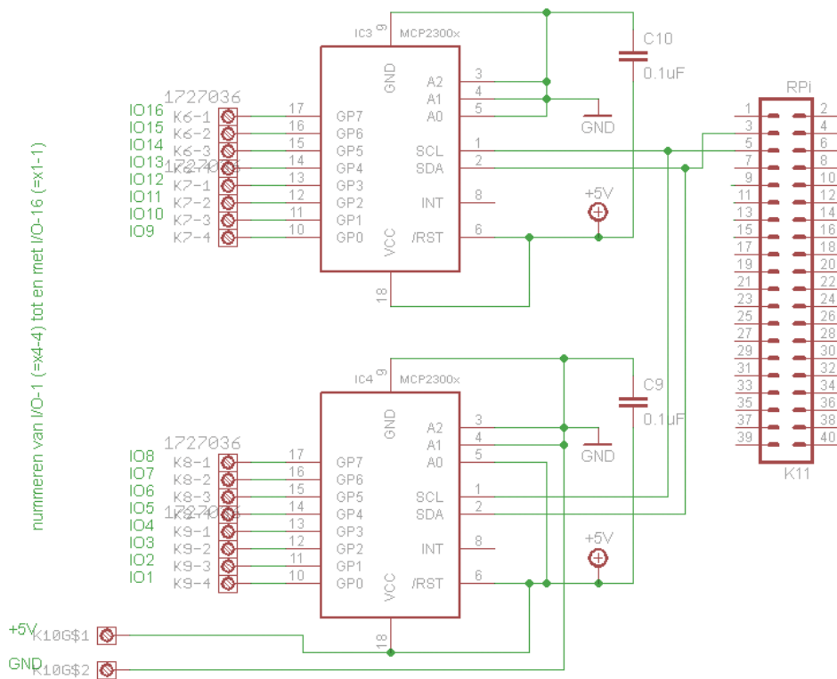
Figure 14.5. LEGO Raspberry Pi board I 2 C I/O.
