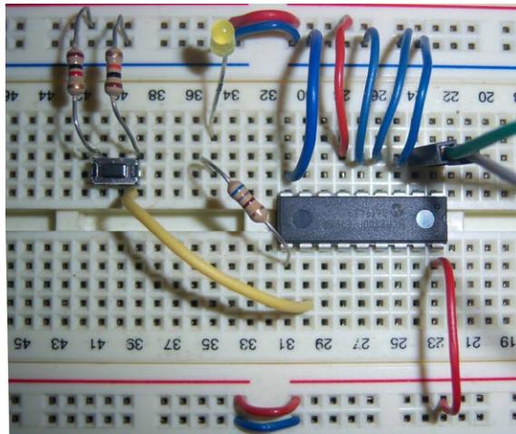
Figure 9.8. Setup on the breadboard.
