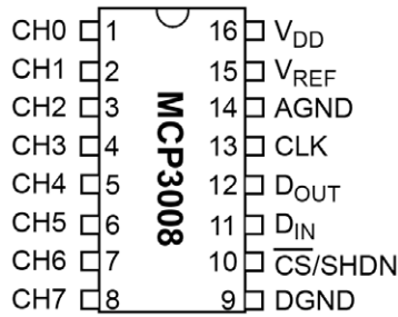
Figure 12.8. Pinout for the MCP3008.
