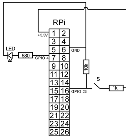
Figure 12.1. Connecting the LED to the header.
