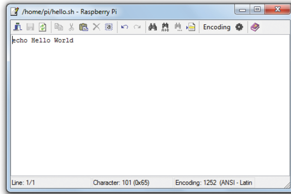
Figure 4.5. WinSCP editor.
