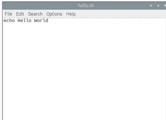
Figure 4.3. Text Editor
