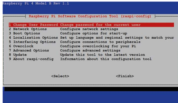
Figure 3.7 Enable SSH
