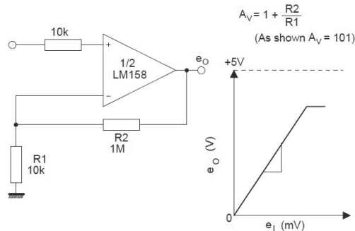
Figure 8.8. Non-inverting DC amplifier circuit. 57
