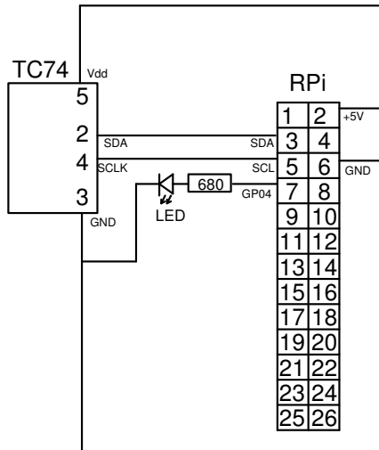
Figure 11.17. Connecting the TC74 and a local alarm LED.
