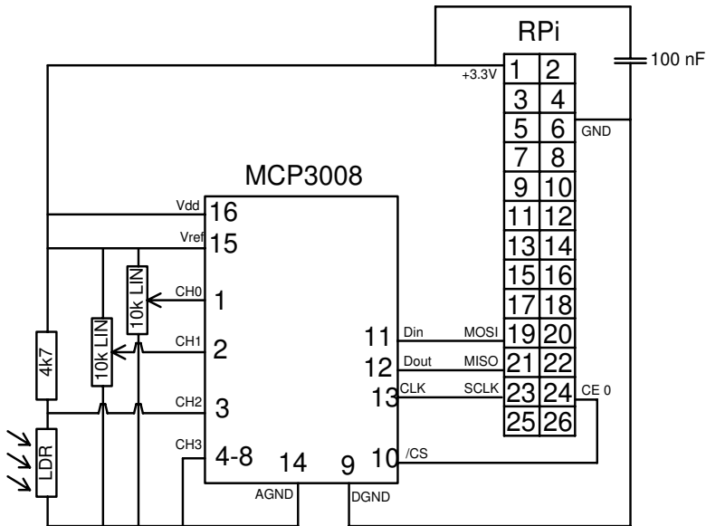
Figure 12.9. Connecting an LDR and two potentiometers.
