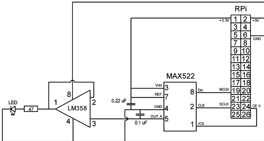
Figure 8.11. MAX522 with LM358 opamp.
