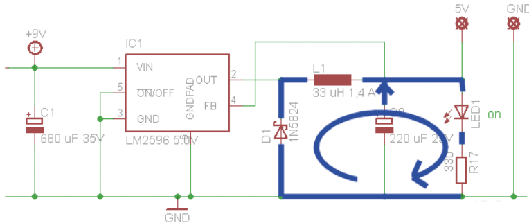
Figure 14.4. Buck converter: flywheel winding down.
