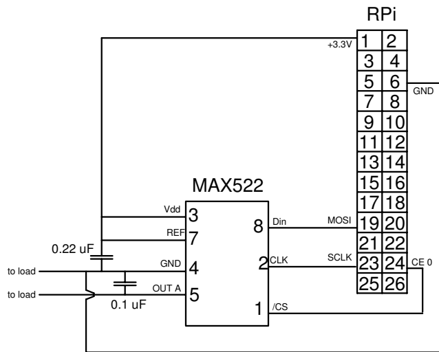
Figure 12.3. Connecting the MAX522 to the header.
