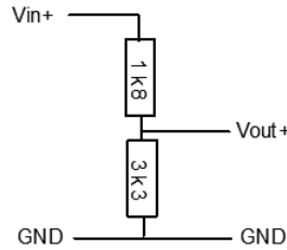
Figure 10.5. Potential divider: from 5 ( V_{in+} ) to 3.3 V ( V_{out+} ).
