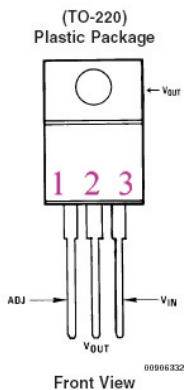
Figure A.2. Pinout for the LM317.
