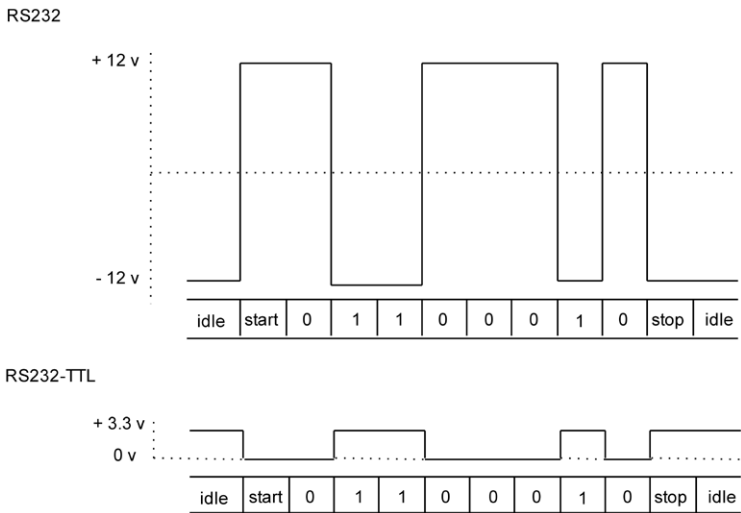
Figure 10.4. Transmitting the letter b using RS232 and RS232-TTL
